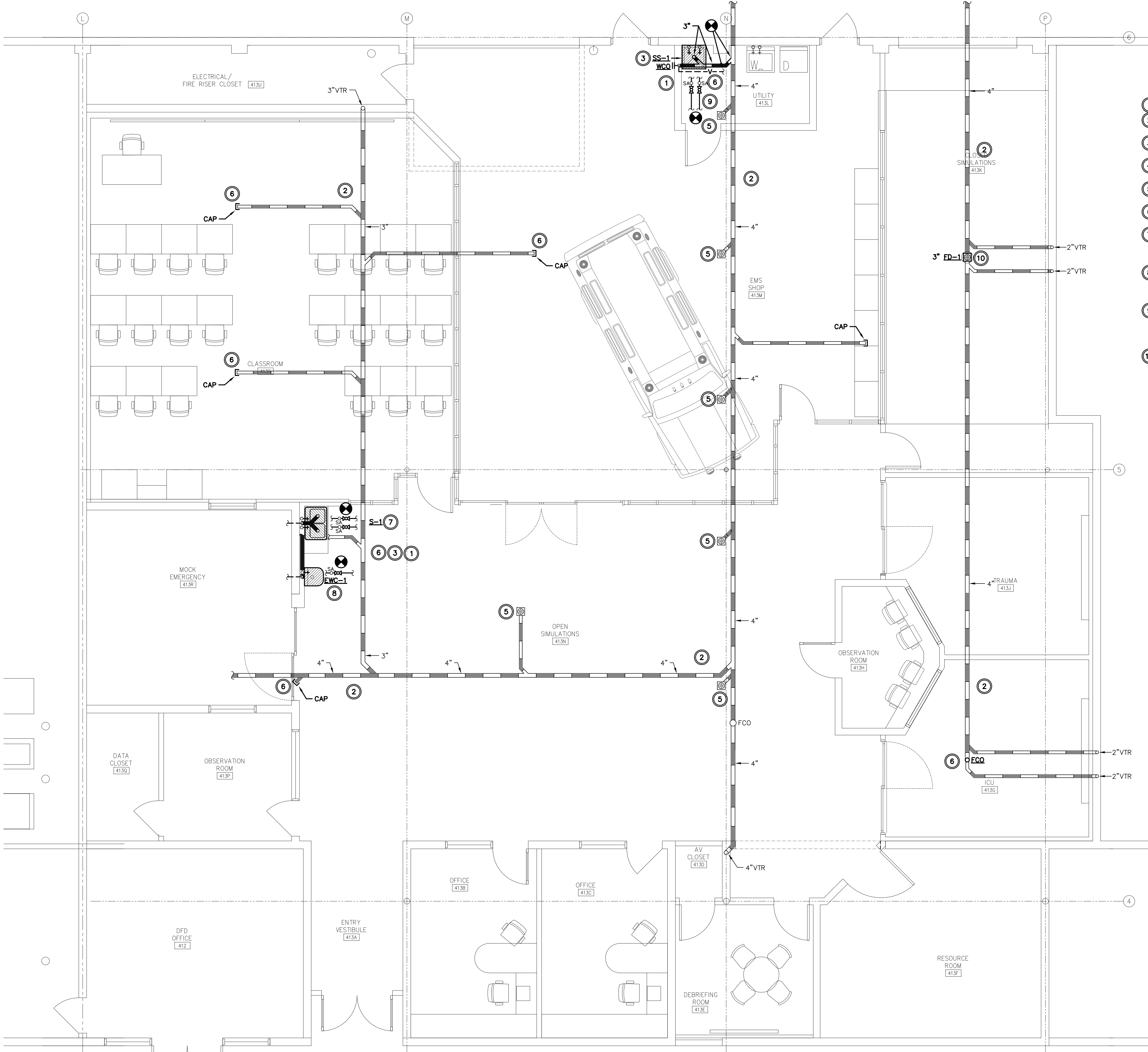
1 PARTIAL FIRST FLOOR - PLUMBING PLAN
