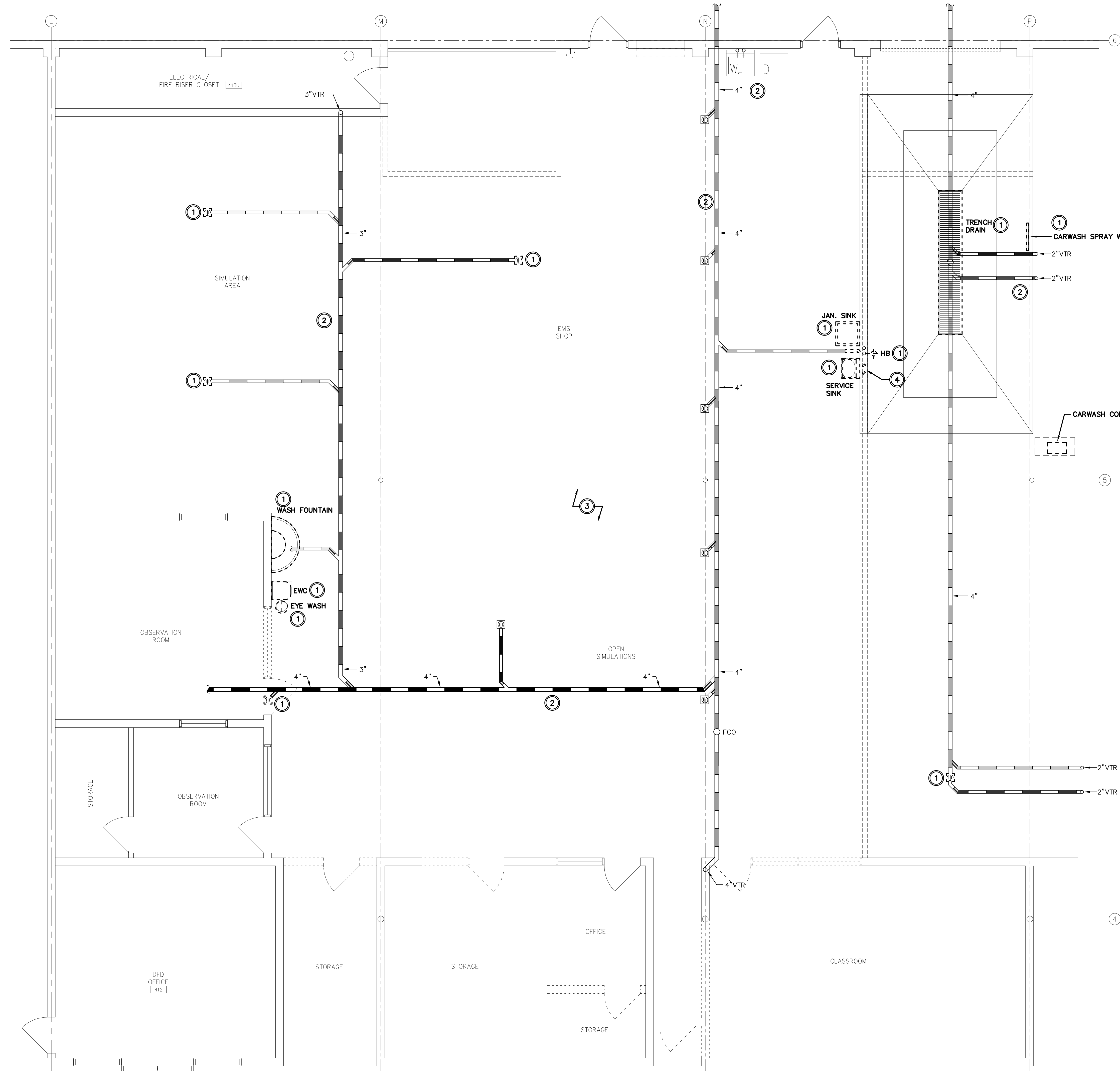
① PARTIAL FIRST FLOOR - PLUMBING DEMOLITION PLAN
