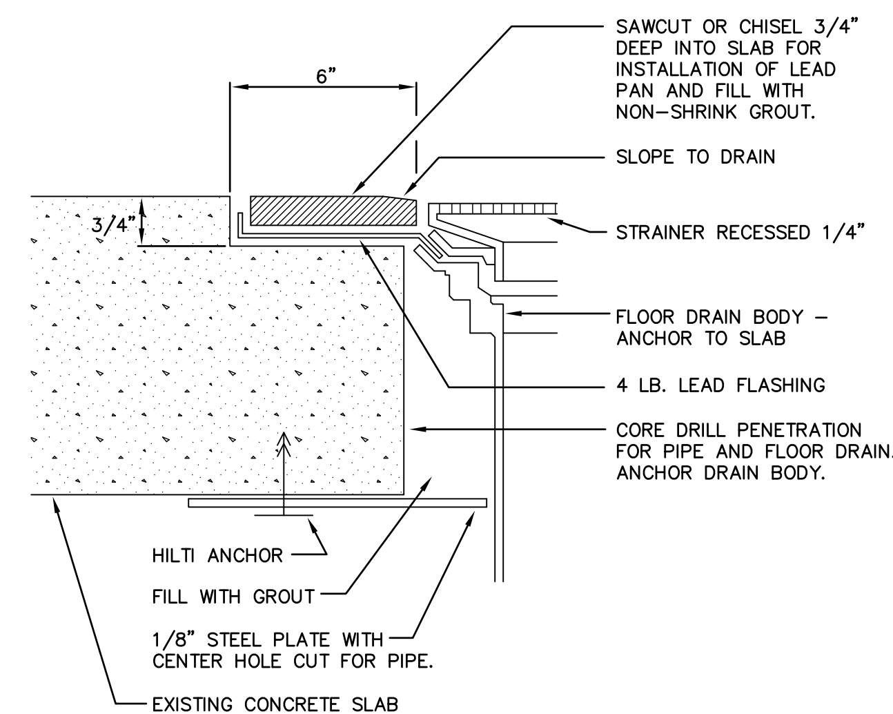
1 DRAIN INSTALLATION DETAIL IN EXISTING SLAB NO SCALE
